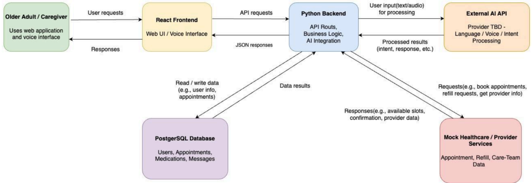
Figure 3. High-level system architecture and integration boundaries.
